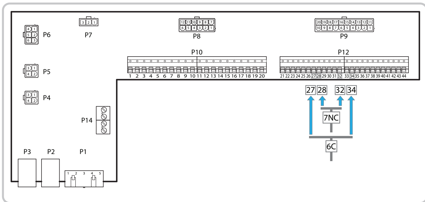
Main circuit CS2000, CS2500 and CS2500 V2.
