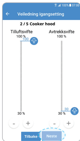
Side 2/5 Luftmengder, COOKER HOOD
