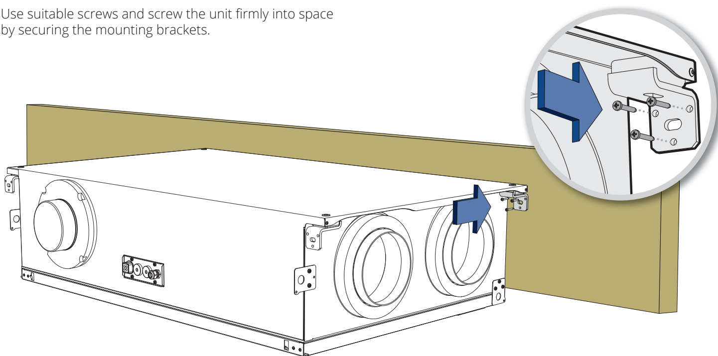
Figure 10 Side mounting
