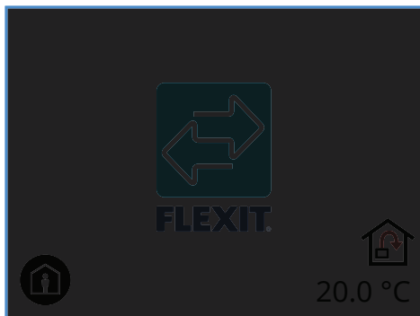
Screensaver 2
